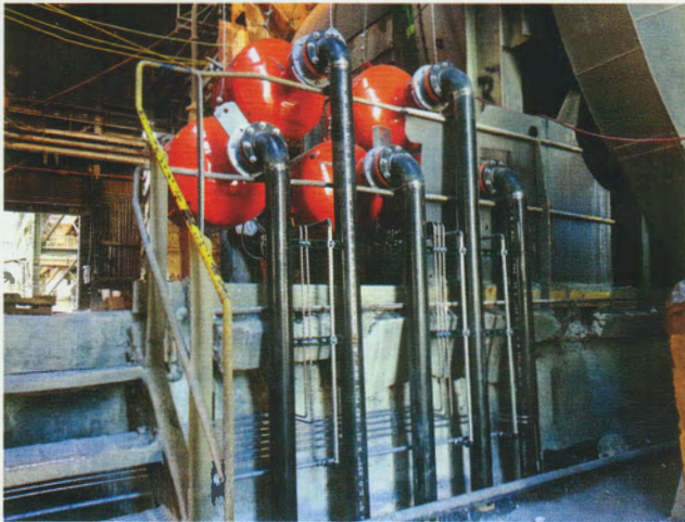
4.5 in. (11.5 mm) pipes lead down to holes drilled into the concrete floor, then continue under the subfloor.
